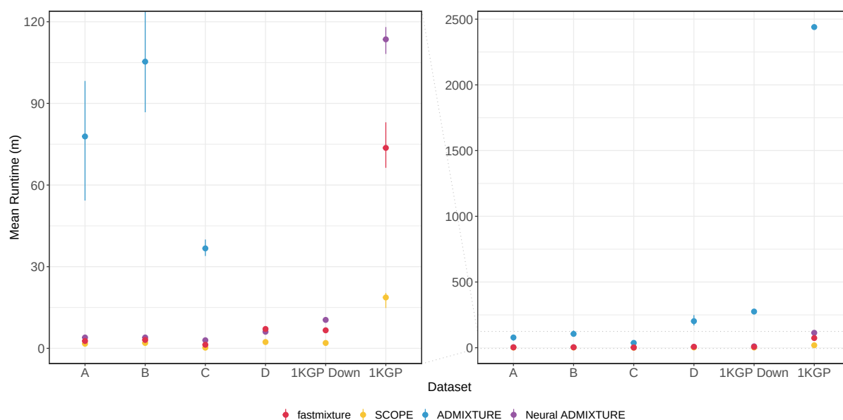
Figure 3 – Runtime (in minutes) for the different software measured across five runs in the four simulated scenarios (A, B, C, and D), and in the two 1000 Genomes Project datasets: one including all individuals (1KGP), and the downsampled dataset (1KGP Down). The intervals display the full range of runtimes across the six runs. On the left, a zoomed-in version highlights the runtime differences between the software with more similar times. The results are also described in Table S1. All analyses have been performed on a cluster with an Intel(R) Xeon(R) Gold 6152 CPU using 64 threads.
